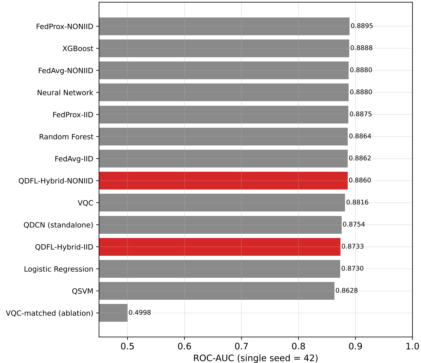
Primary (Azamuke 2024) (red = QDFL variants)
