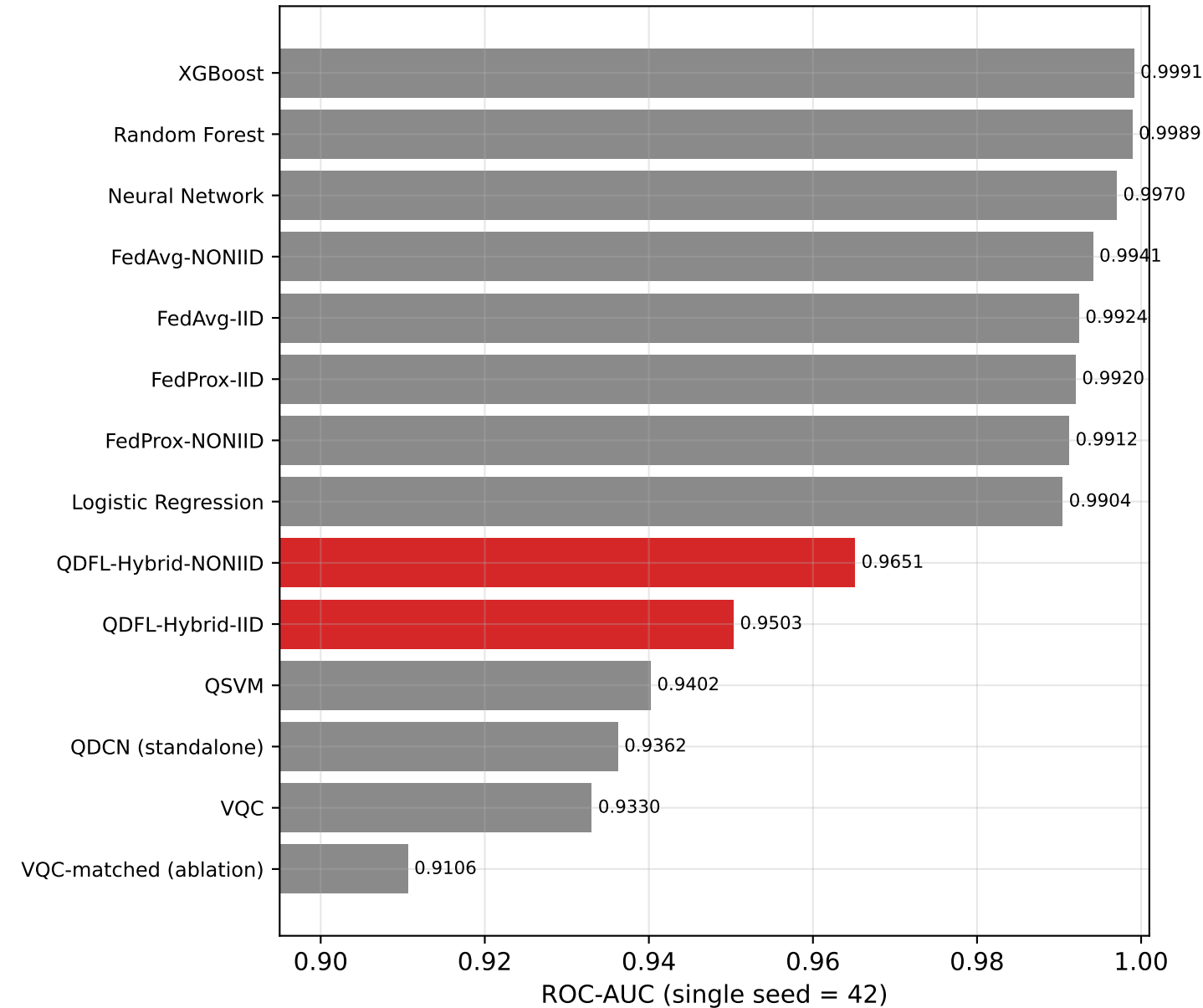
PaySim (Lopez-Rojas) (red = QDFL variants)
